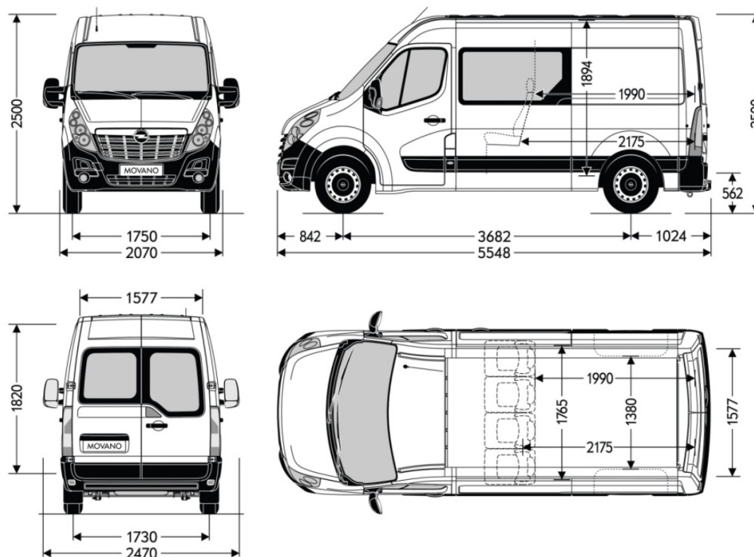
Opel Movano Crew Van FWD L2H2
